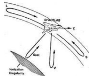
Figure 4(a). Possible echo paths when Spacelab is within an equatorial bubble or duct and when a field-aligned irregularity patch exists below Spacelab
